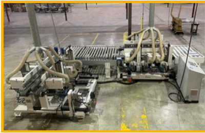
Belino "LF-1000SB" Double Sided Sander – (12) Sanding Heads (2022)
