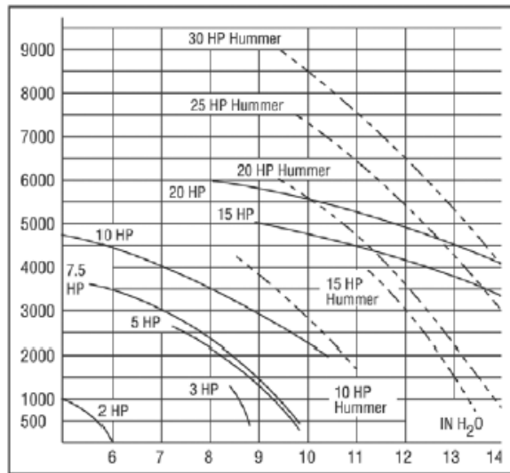
C.F.M. PERFORMANCE CURVES
